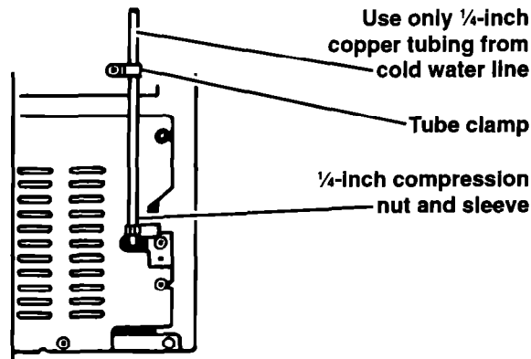
Style #2 valve
